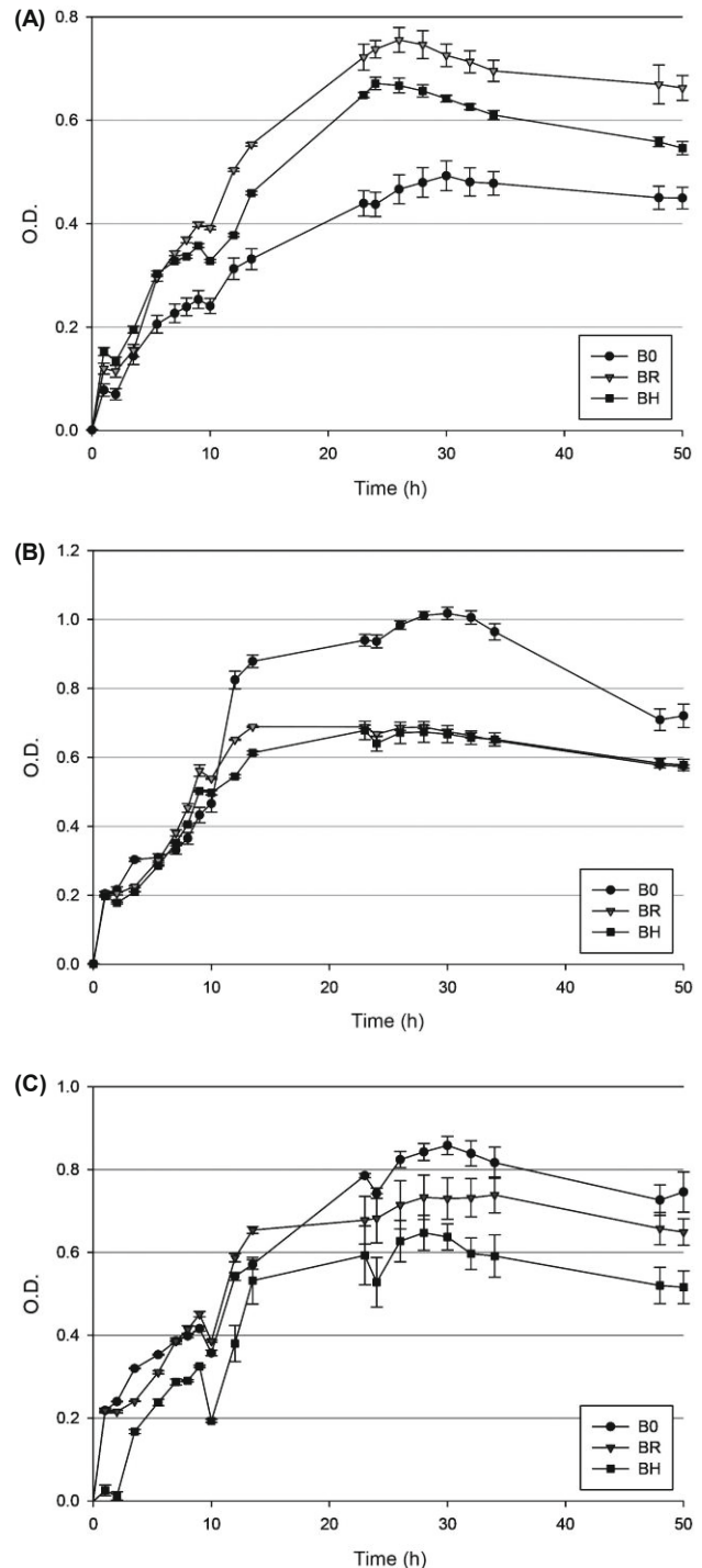
Fig. 1. Growth curves of three laboratory culture bacteria under static magnetic field. (A) Escherichia coli , (B) Pseudomonas aeruginosa , and (C). Staphylococcus epidermidis . Error bars represent 1 standard error with triplicates.
