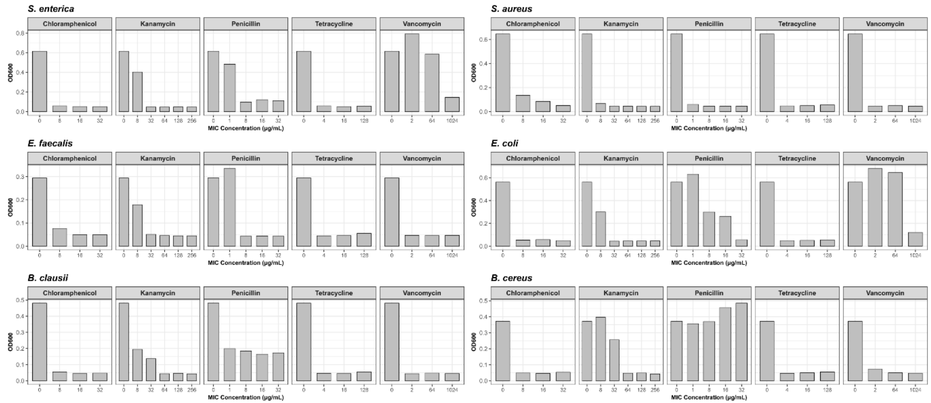
Fig. S2. MIC profiles of quality control strains under 2% NaCl conditions.
