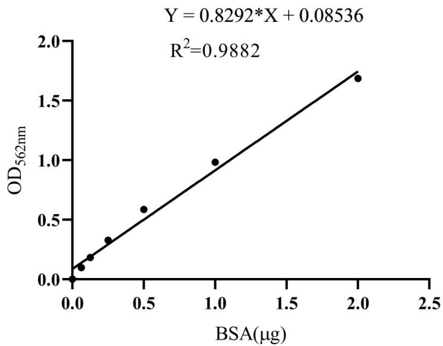
Fig. S7. The protein assay standard curve for BCA.
