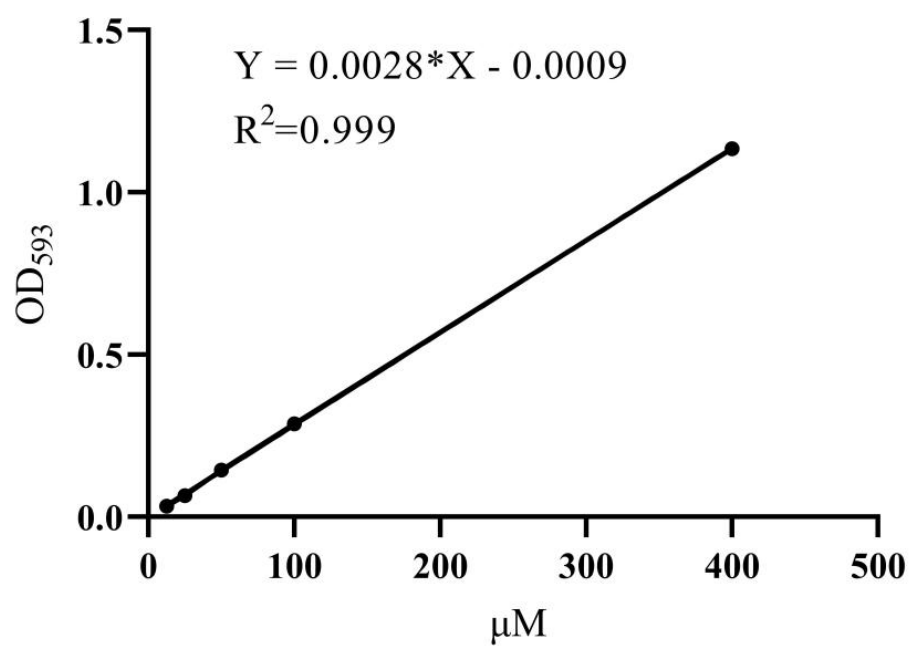
Fig.S6. Linear relationship between iron concentration and OD 593 .
