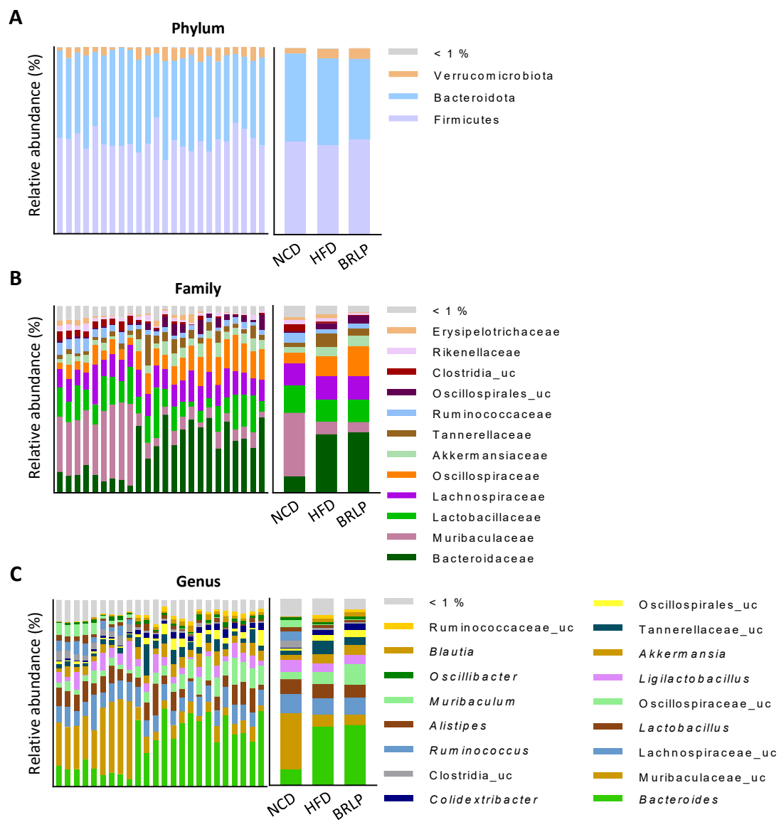
Fig. S2. The stacked box plots of taxonomic composition at the (A) phylum, (B) family, and (C) genus level. Data are presented as mean of relative abundance.
