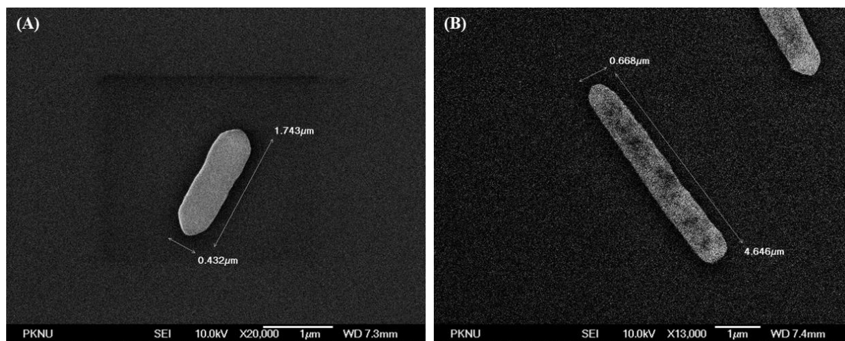
Fig. S3. Scanning electron micrograph of strains FM7315 T (A) and FM7330 T (B) cells. Bar, \mu\text{m} .
