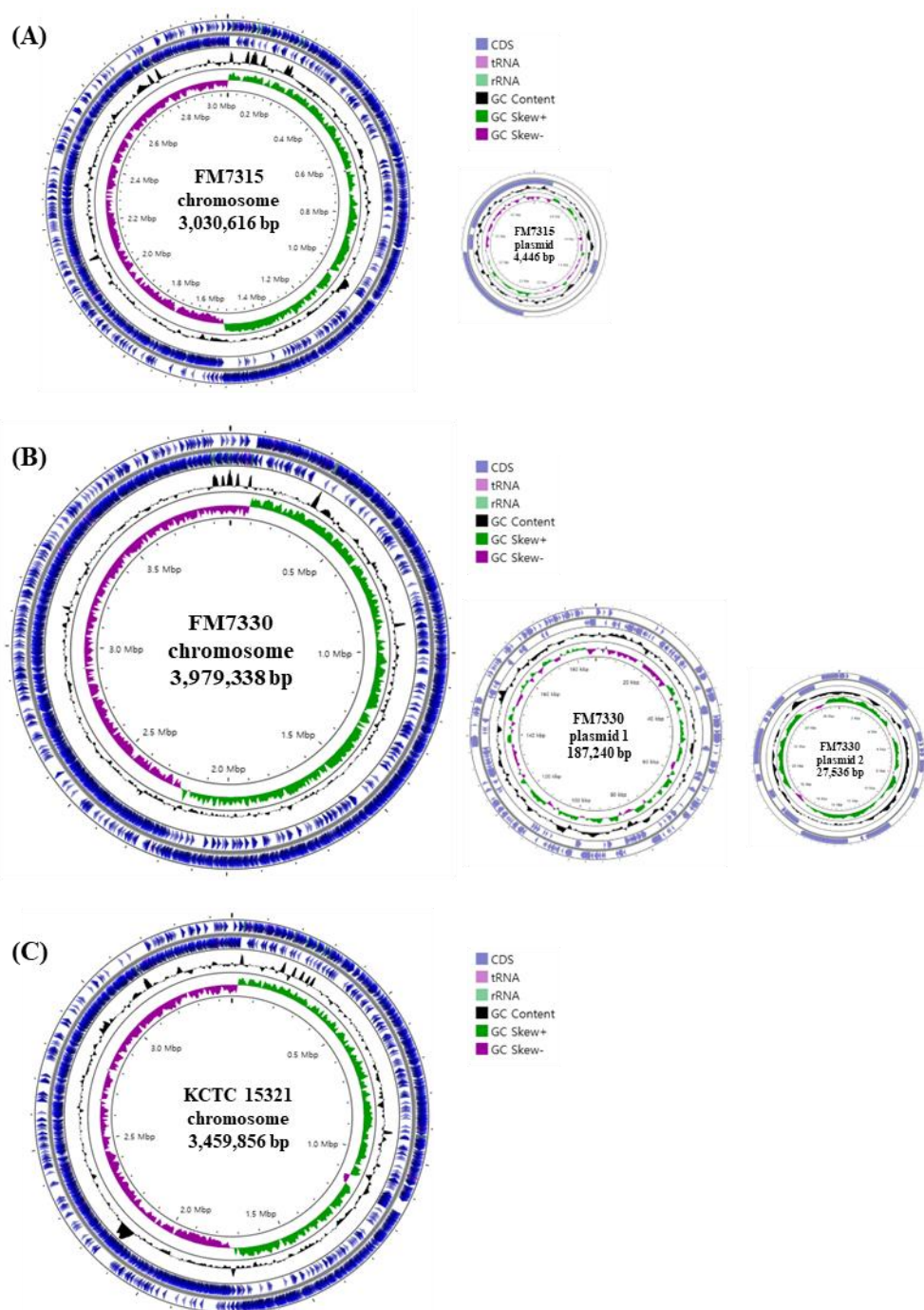
Fig. S2. Genome maps for strains H. sporogenes FM7315 T (A), H. myeolchijeotgali FM7330 T (B), and H. lingqiaonensis KCTC 15321 T (C).
